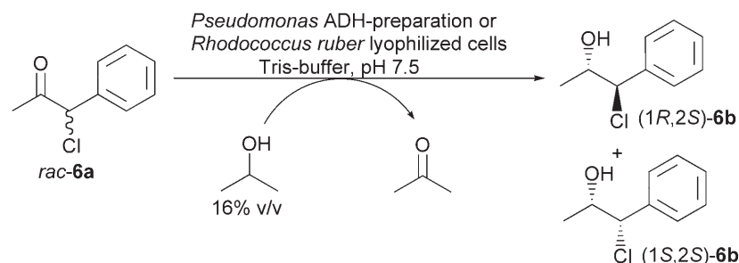
Scheme 2. Diastereoselective reduction of rac - 6a .
