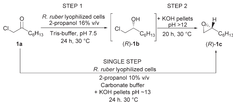
Scheme 3. “One pot-two steps” and “one-pot-one-step” transformation of \alpha -chloro-ketone to the corresponding epoxide by biocatalytic hydrogen-transfer reduction followed by base-mediated ring closure.
