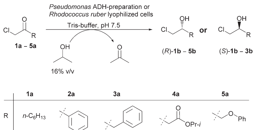
Scheme 1. Biocatalytic reduction of \alpha -chloro-ketones via hydrogen transfer to access ( R )- or ( S )-halohydrins.
